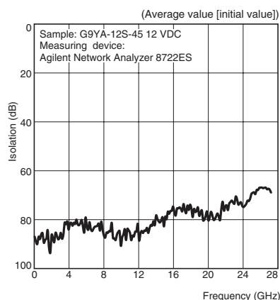
High-frequency Characteristics (Isolation) (See notes 1 and 2.)
