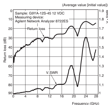
High-frequency Characteristics (Return Loss, V.SWR) (See notes 1 and 2.)
